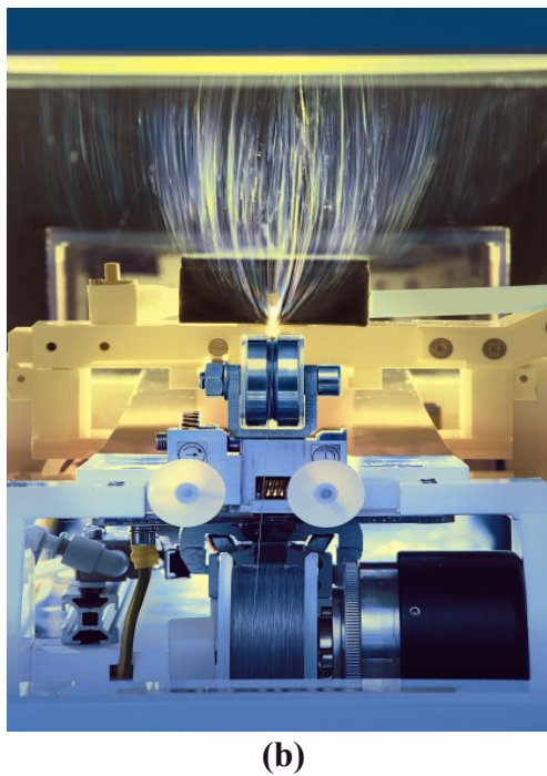
Figure 9. (a) Commercial unit for roller based needleless electrospinning (16) . (b) Commercial unit for free surface wire based needleless electrospinning (21) .
