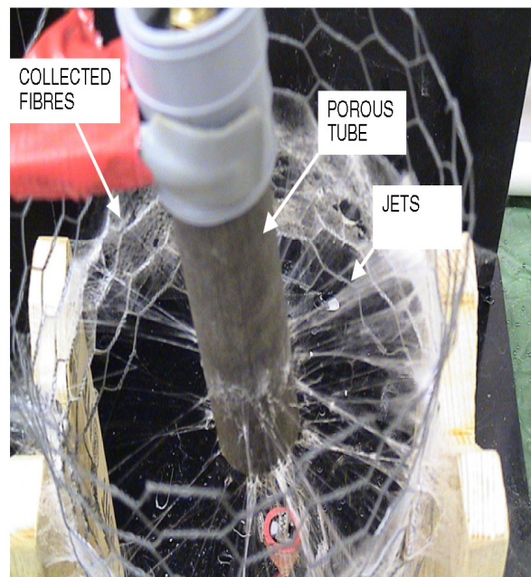
Figure 7. Proof of concept apparatus for hollow tube electrospinning (13) .
